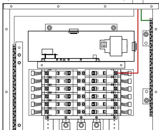
Benjamin ArcLight Panel (remote controllable circuit breakers)
